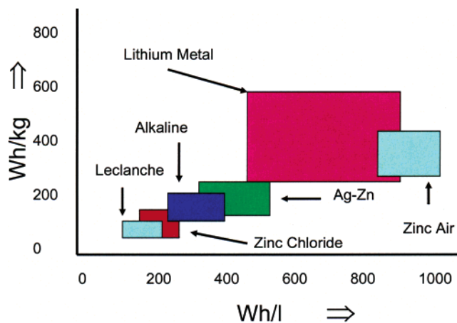
Figure 13. Energy storage capability of common primary battery systems.
